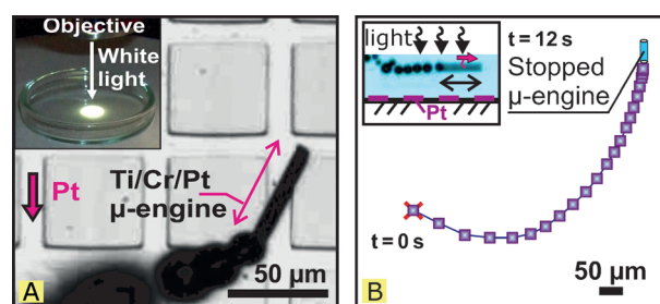
Figure 1. A) Optical image of a self-propelled Ti/Cr/Pt \mu -engine moving above a platinum-patterned silicon surface. Inset: local illumination of the fuel solution containing the \mu -engines. B) Tracked trajectory of a \mu -engine stopped after 12 s of illumination above a Pt-patterned Si surface. The time interval between two spots in the plot is 0.5 s. Inset: optical image of the mobile \mu -engines self-propelled above the patterned surface. See also Video S1 in Supporting Information.
